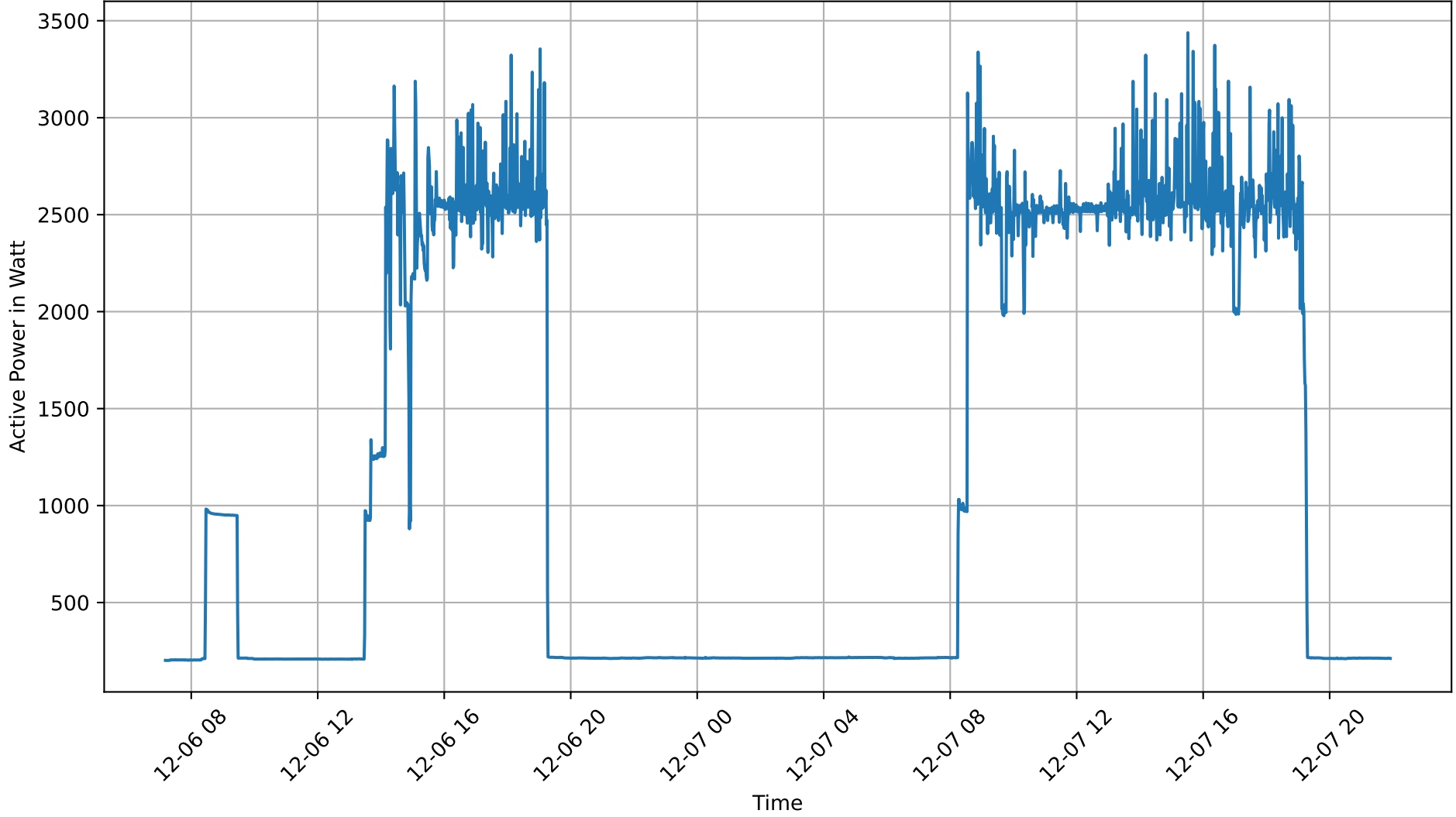
Active power consumption of the EMAG VLC 100 Y vertical lathe
